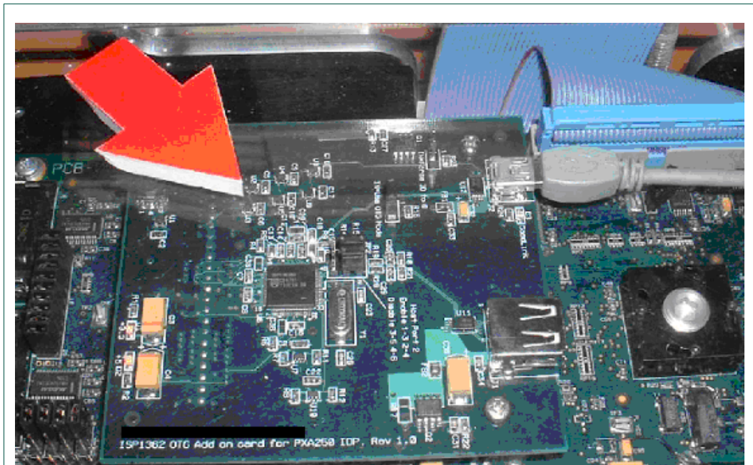
Fig 8. ISP1362 OTG add-on card on the PXA250/255 IDP
